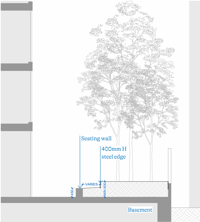
NORTHERN COURTYARD SECTION (A-A)
