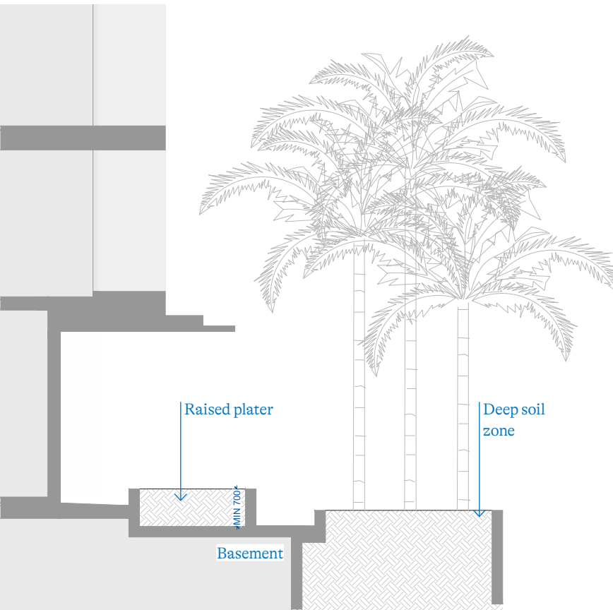
ENTRY PLANTER SECTION (C-C)
