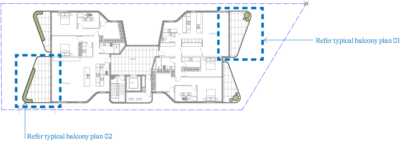
LEVEL 4
