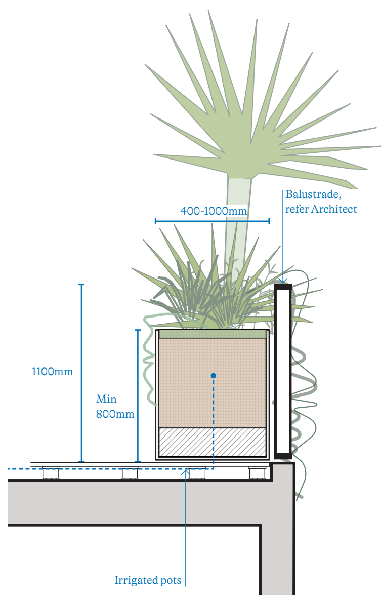
TYPICAL BALCONY SECTION
