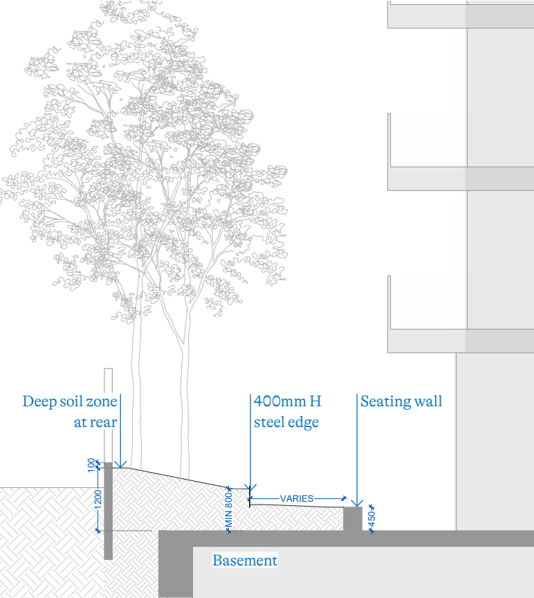
REAR COURTYARD SECTION (B-B)
