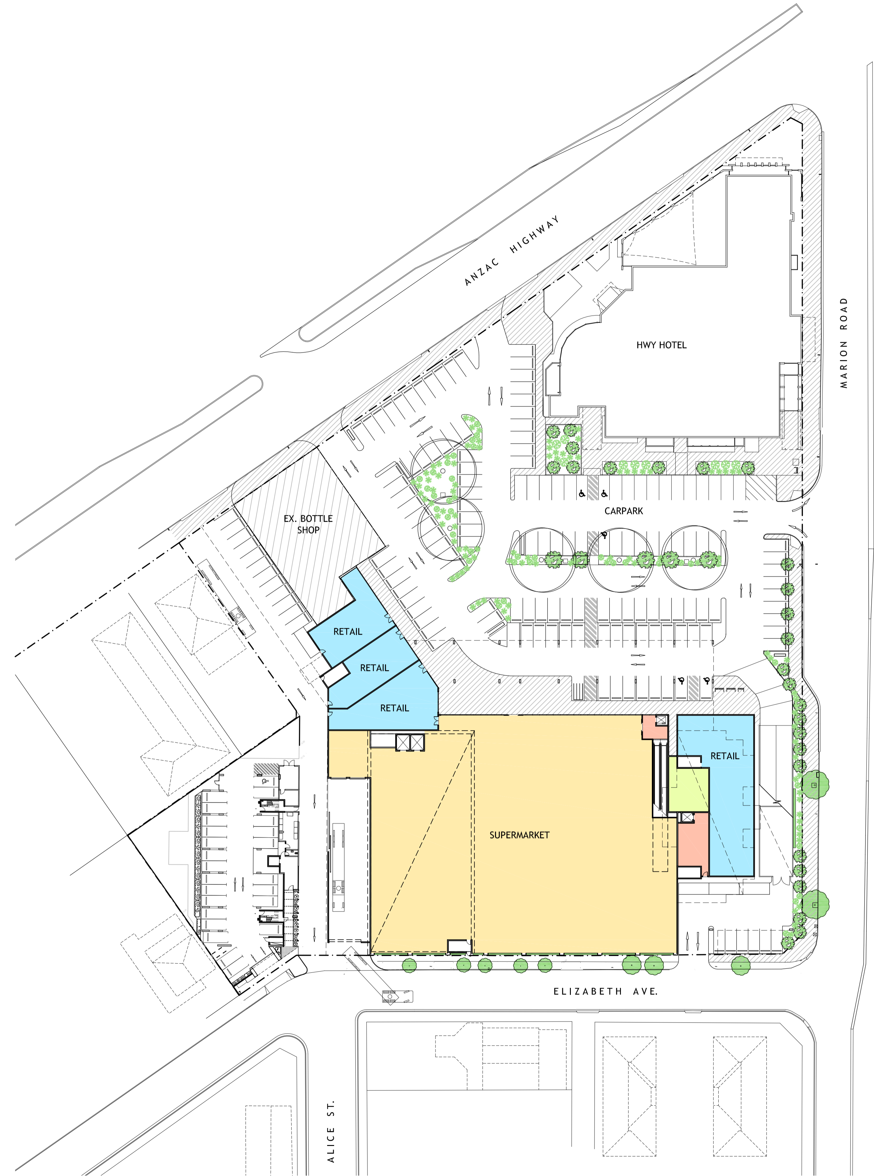
SITE PLAN SCALE 1:500 @ A1 (1:1000 @ A3)
