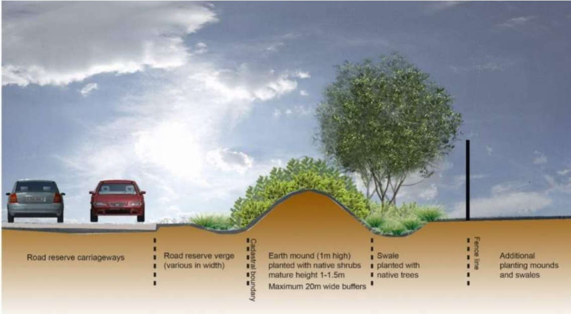
Typical buffer and mound landscape treatment cross section Note: Drawing is not to scale. It is a concept only and will require detailed landscape design to confirm
