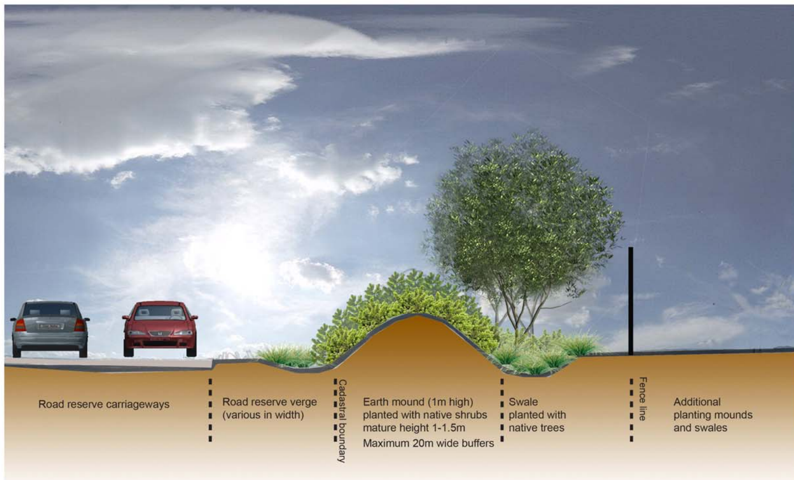
Typical buffer and mound landscape treatment cross section
