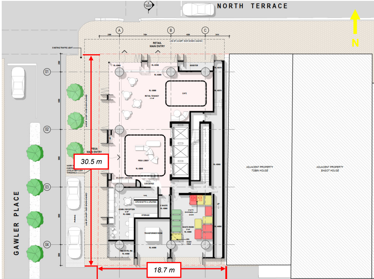
Figure 5: Ground floor plans with the plan-form dimensions overlaid.
