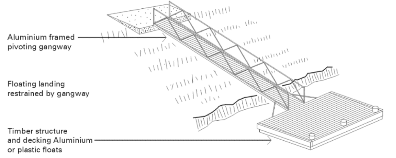
Figure 3 - Floating pontoon (cross-section)
