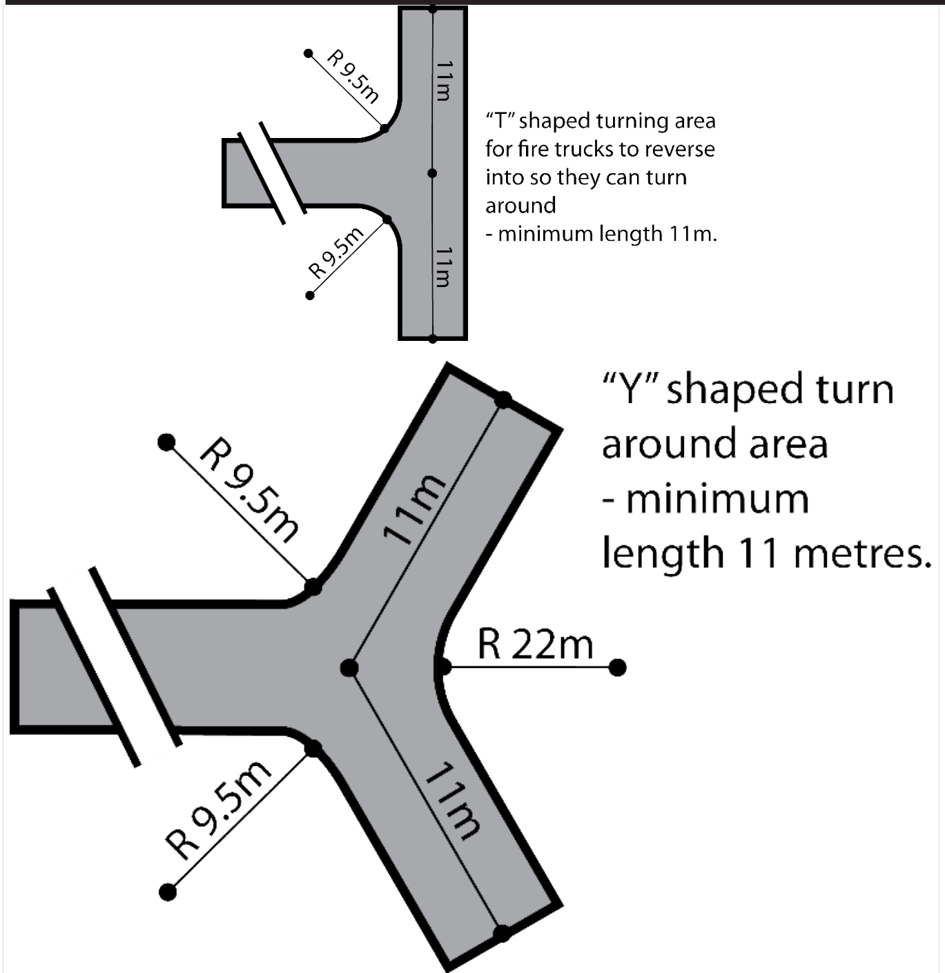
Figure 5 - Driveway Passing Bays
