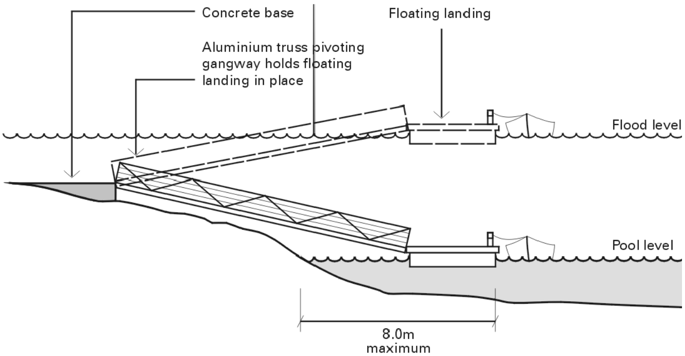
Figure 4 - Jetty
